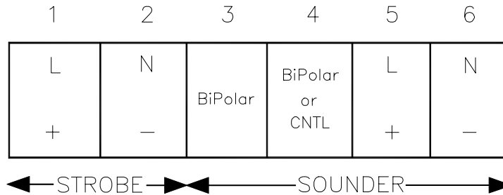
WIRING DETAILS FOR YL UNITS
