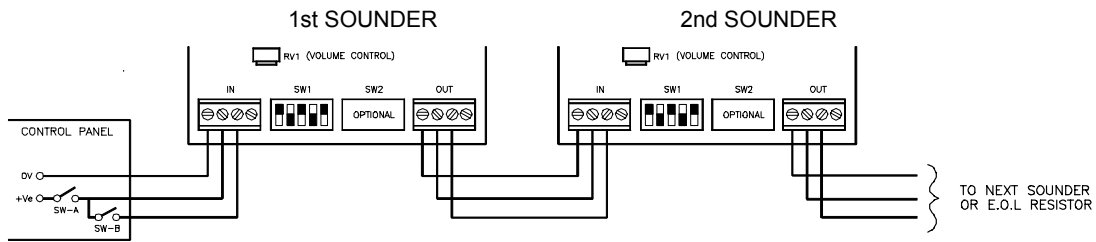
WIRING DETAILS FOR YL UNITS
