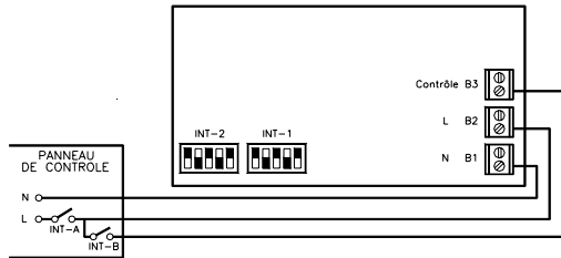
FIGURE 4: BRANCHEMENT DU SYSTEME
